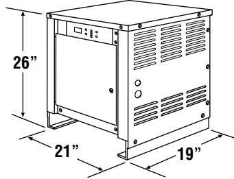
Single Phase
